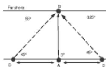
Original observation from A to B reveals 0 azimuth. Move toward either C or D. When the azimuth is 45 degrees different, the distance AC or AD equals AB (the river's width).
