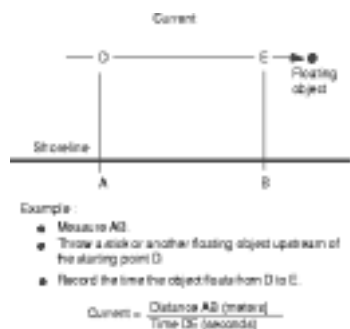
Figure 7-2. Measuring the current's velocity
