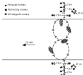
Figure 7-12. Centerline marking and operation
